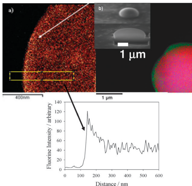
Fig. 4 TEM-EDX element map and image for polymer particles: (a) cross-sectional map showing fluoropolymer distribution (fluorine map) across a section of a particle and the subsequent histogram over the area within the yellow box; (b) showing elemental distribution around an intact particle (red—carbon, pink—oxygen, and green—fluorine). The inset shows an SEM image of a single particle before and after focussed ion beam slicing to yield ~300 nm cross-sectioned slice. The fluorine-rich halo is present in all images.
