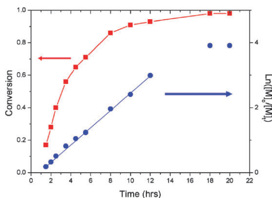
Fig. 1 Conversion as a function of polymerisation time and pseudo-first-order kinetic plot for polymerisation of MMA via macro-RAFT agent in scCO 2 .
