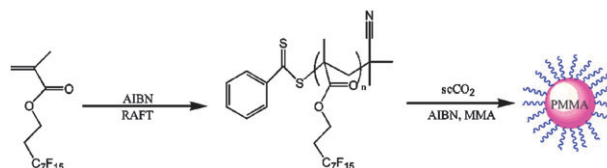
Scheme 1 Synthetic route for PMMA particles by macro-RAFT agent.
