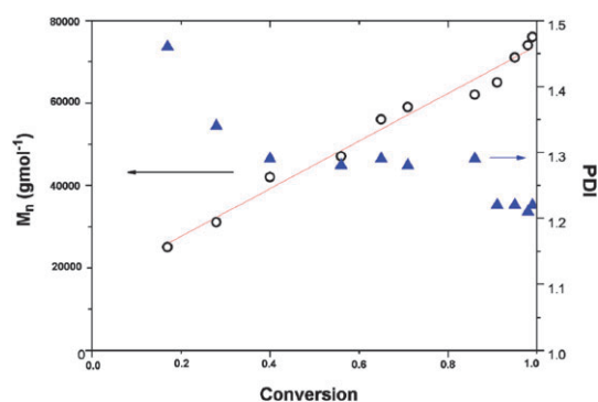
Fig. 2 Molecular weight evolution and molecular weight distribution with monomer conversion for MMA showing excellent linear evolution and the expected narrowing of the PDI at higher conversions. Note also that the plot of molecular weight with conversion intercepts the y abscissa at 15 kDa; the molecular weight of the PFOMA surfactant as calculated by 1 H NMR.
